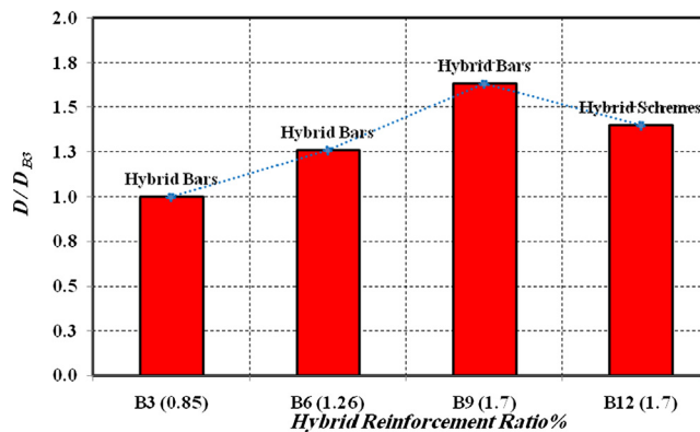
Fig. 29. Effect of Hybrid Reinforcement ratio on the Flexural Rigidity.
