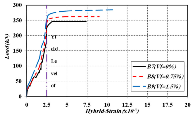
Fig. 16. Load-Hybrid Strain of the Tested Beams for Group C.
