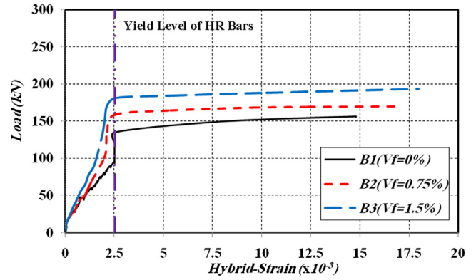
Fig. 14. Load-Hybrid Strain of the Tested Beams for Group A.
